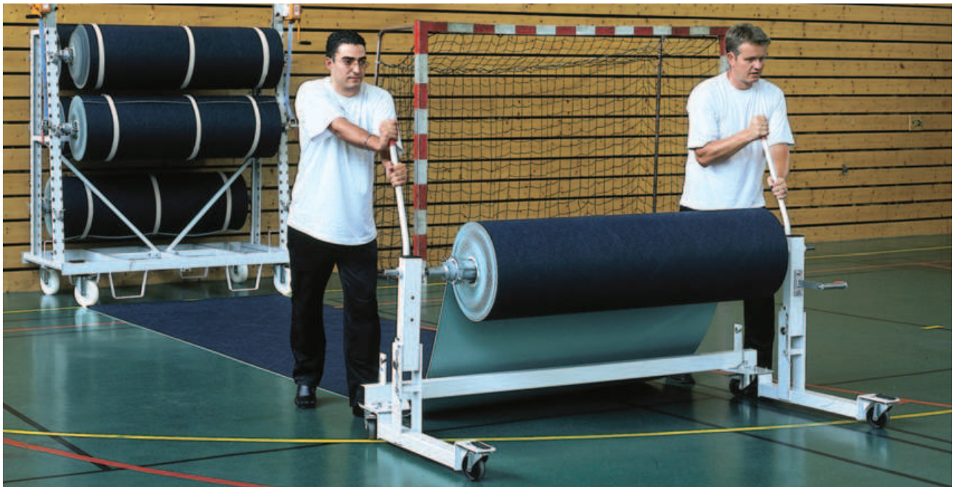
On- Rolling with the Transport and Unroll Trolley- manual and
